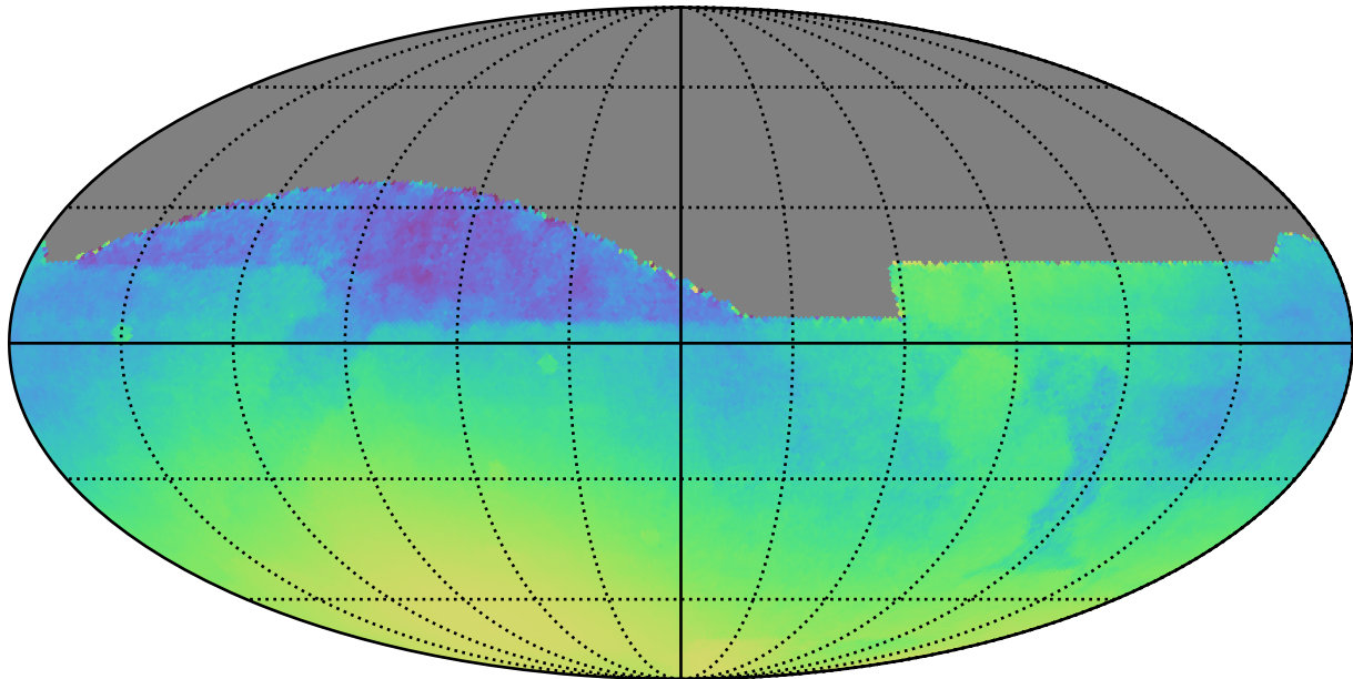
baseline_v3.0_10yrs : Normalized Parallax Uncert @ 22.4
