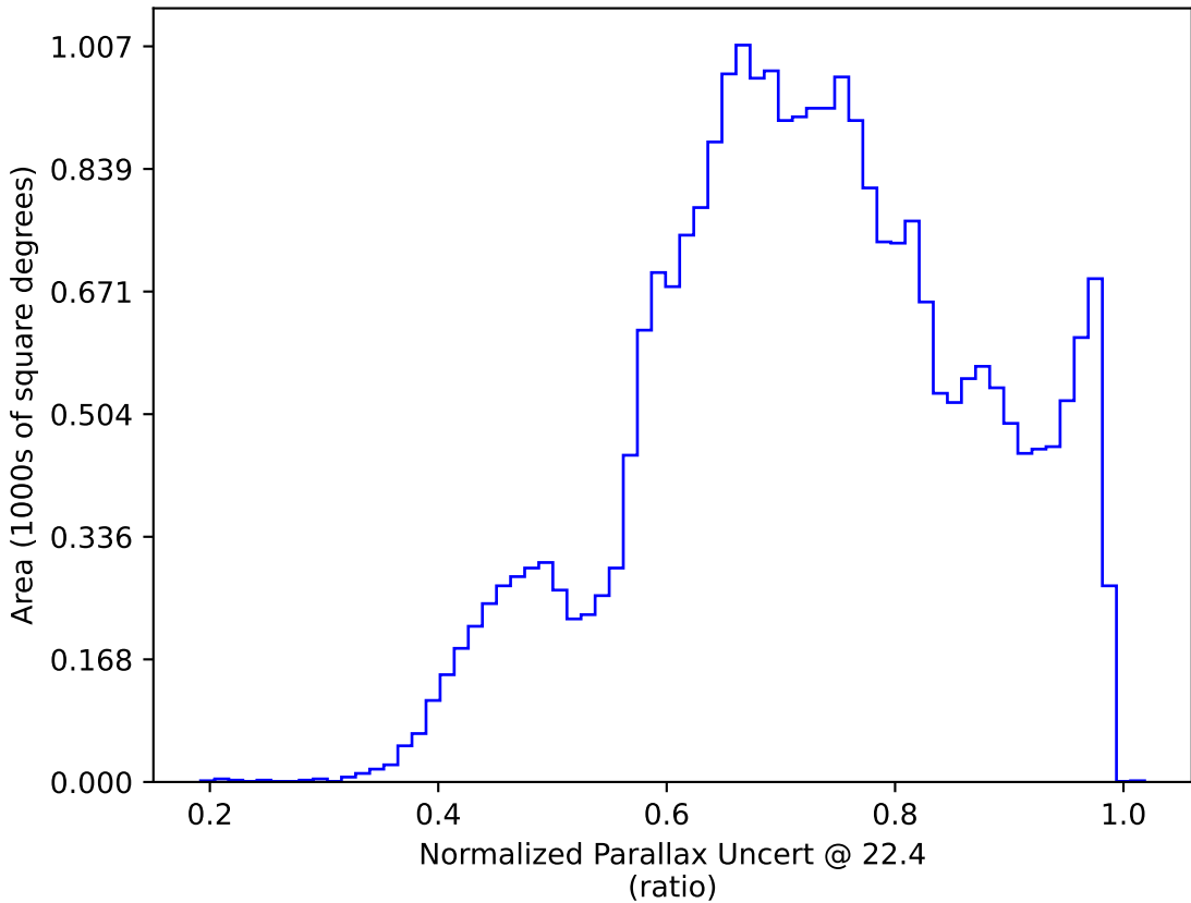
baseline_v3.0_10yrs : Normalized Parallax Uncert @ 22.4
