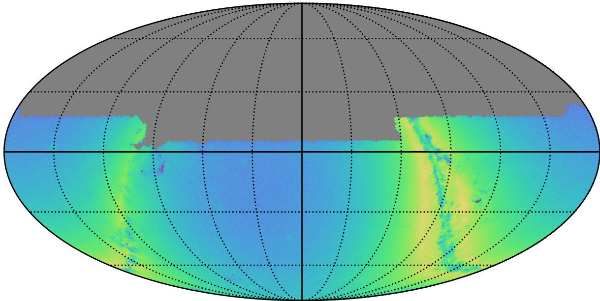
baseline_v3.0_10yrs u: N stars to Precision 0.20
