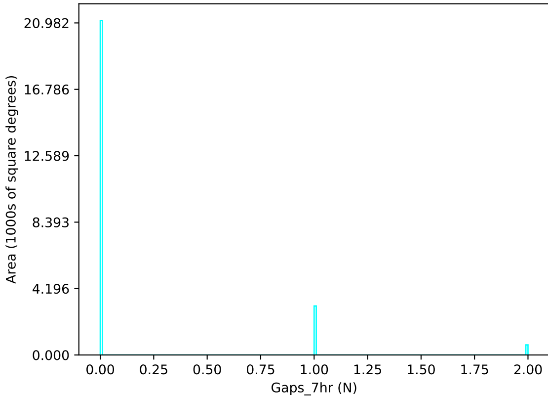
baseline_v3.0_10yrs u band: Gaps_7hr
