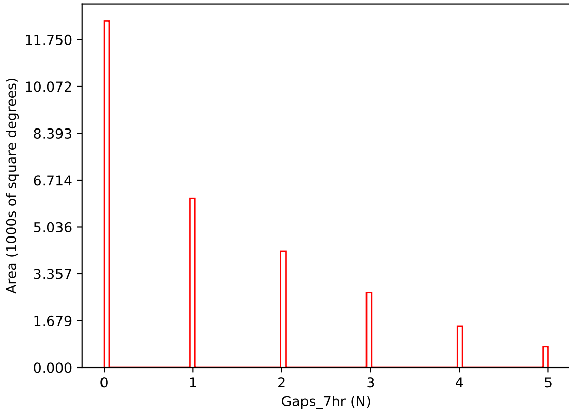
baseline_v3.0_10yrs i band: Gaps_7hr
