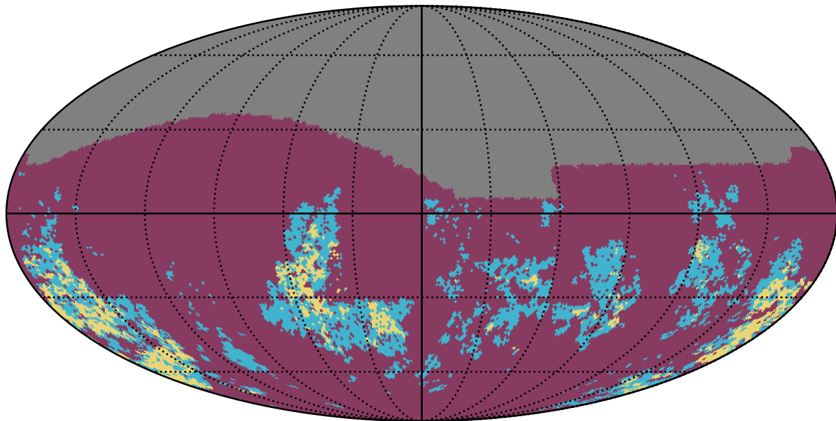
baseline_v3.0_10yrs g band: Gaps_7hr
