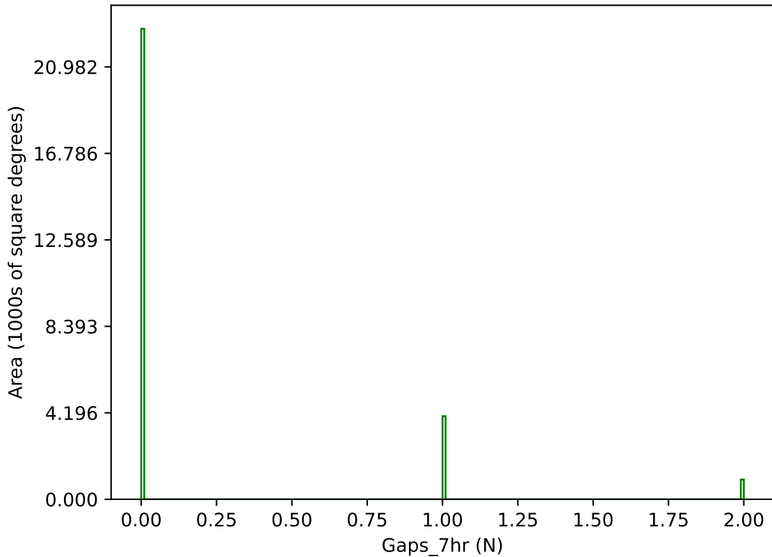
baseline_v3.0_10yrs g band: Gaps_7hr
