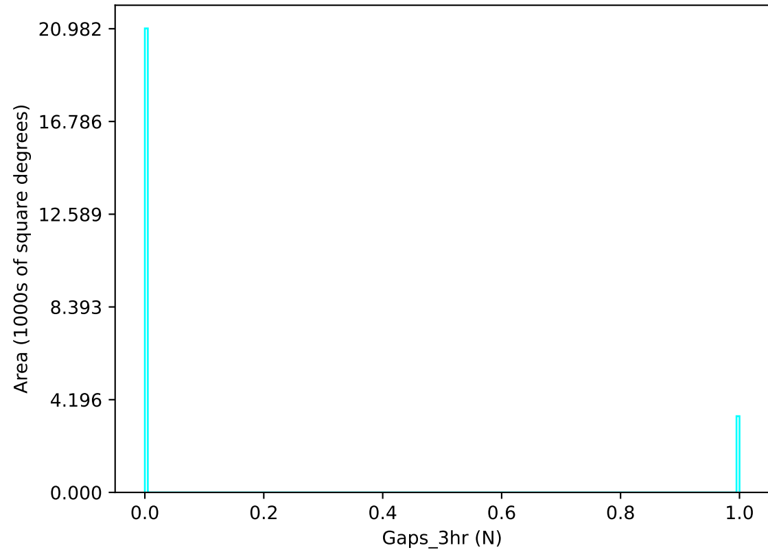
baseline_v3.0_10yrs u band: Gaps_3hr
