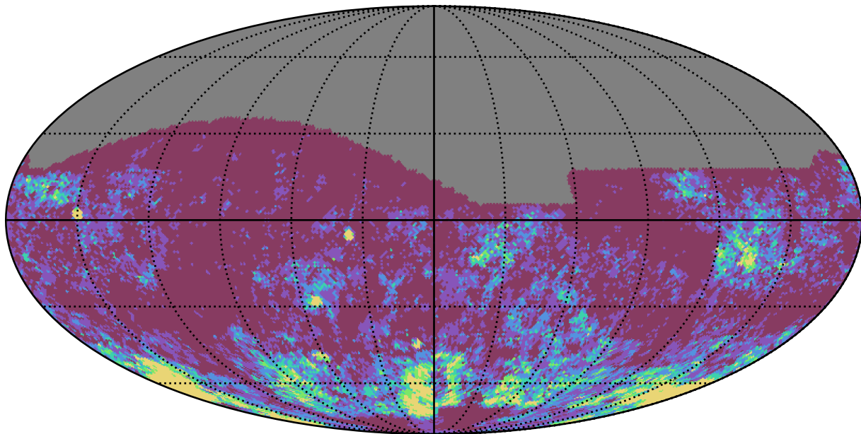
baseline_v3.0_10yrs i band: Gaps_3hr
