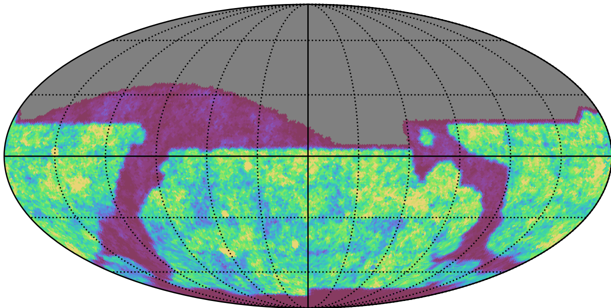
baseline_v3.0_10yrs r band: Gaps_24hr
