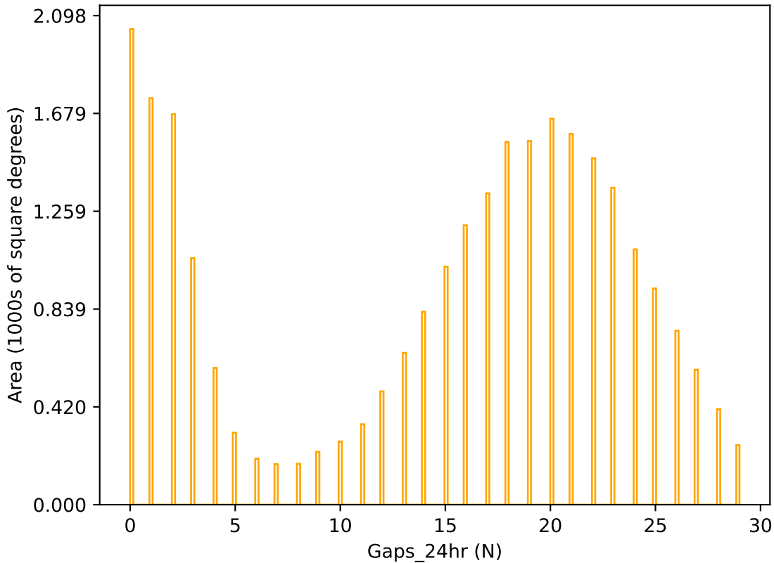
baseline_v3.0_10yrs r band: Gaps_24hr
