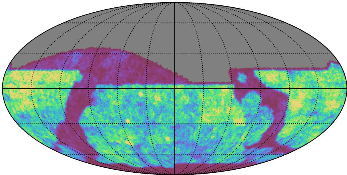
baseline_v3.0_10yrs i band: Gaps_24hr
