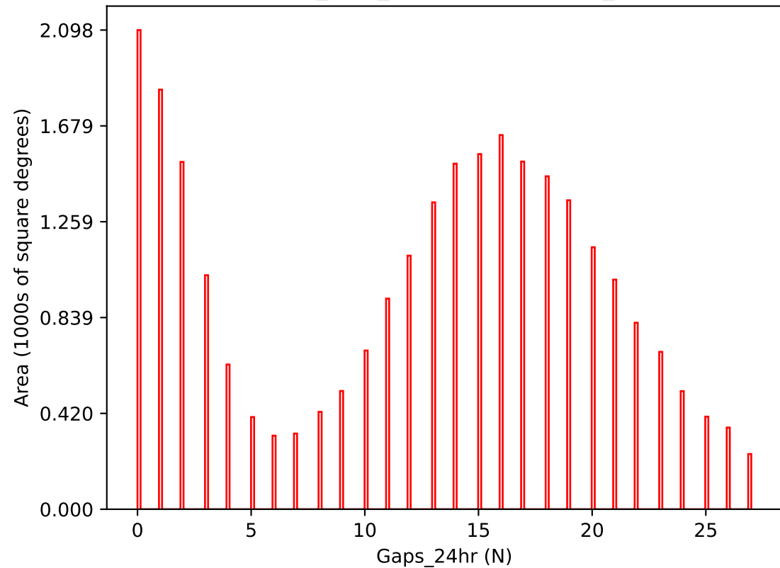
baseline_v3.0_10yrs i band: Gaps_24hr
