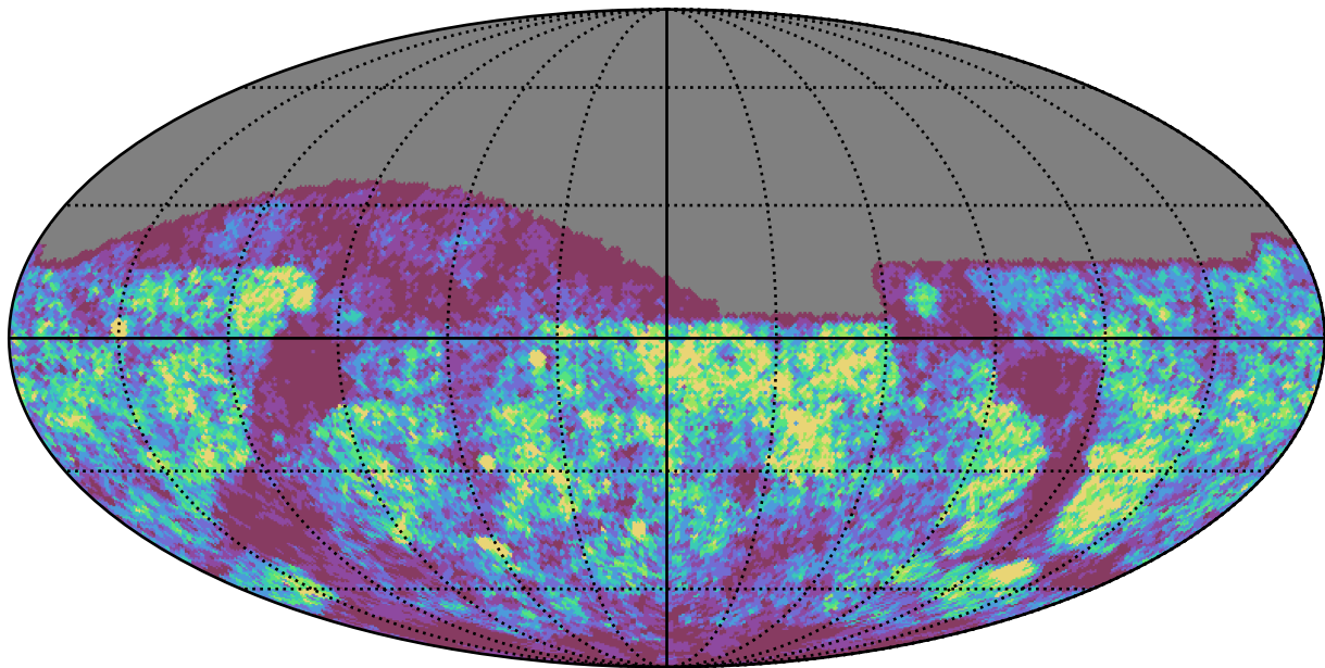
baseline_v3.0_10yrs g band: Gaps_24hr
