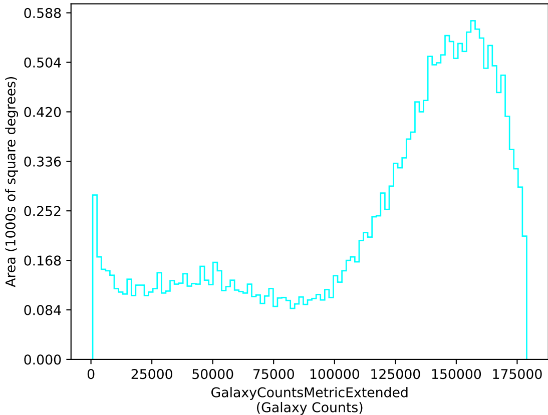
baseline_v3.0_10yrs u: GalaxyCountsMetricExtended
