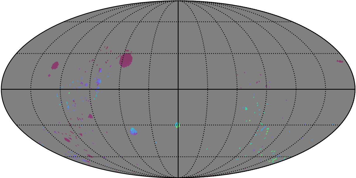
baseline_v3.0_10yrs : GalPlaneSeasonGapsTimescales_open_clusters_map_Tau_55_0
