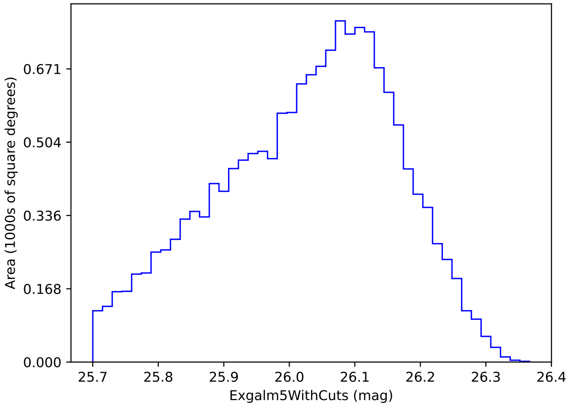
baseline_v3.0_10yrs i band non-DD year 7: ExgalM5WithCuts
