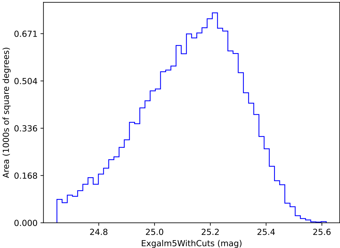
baseline_v3.0_10yrs i band non-DD year 1: ExgalM5WithCuts
