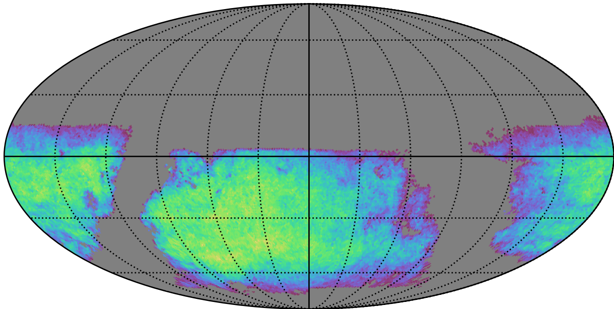
baseline_v3.0_10yrs i band non-DD year 10: ExgalM5WithCuts
