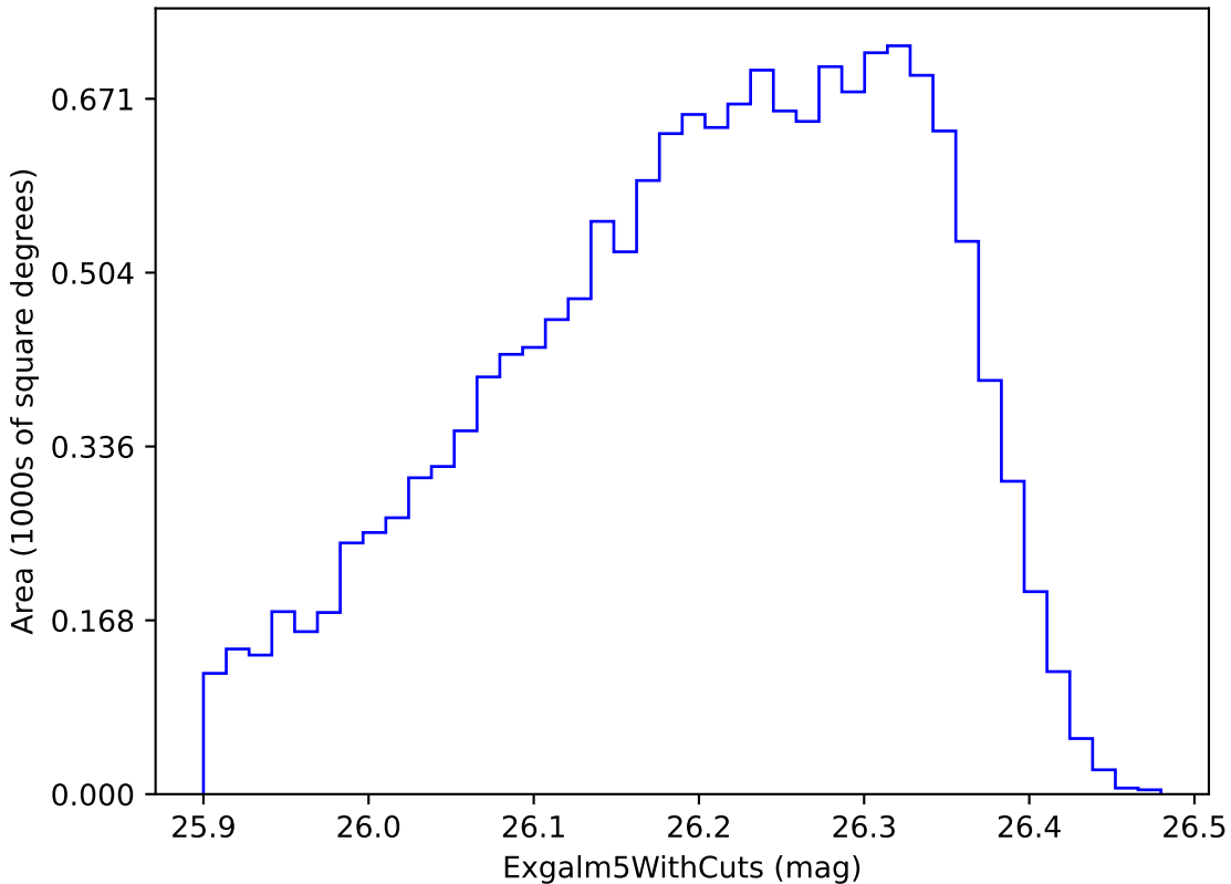
baseline_v3.0_10yrs i band non-DD year 10: ExgalM5WithCuts
