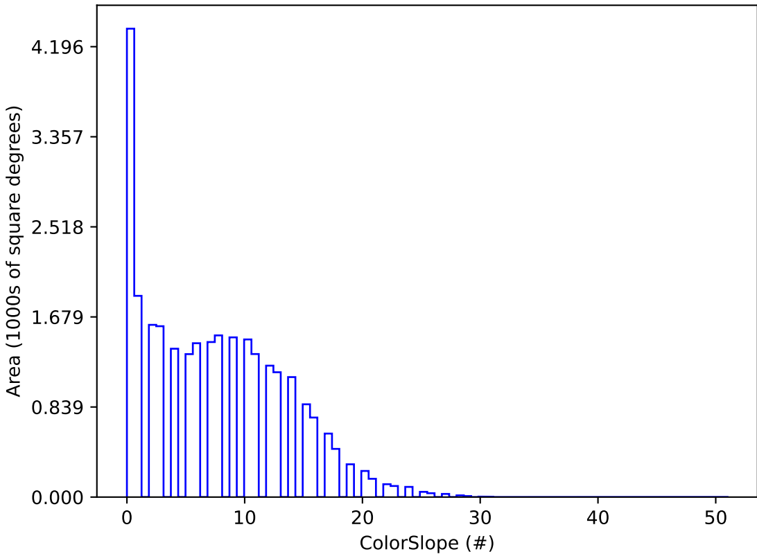
baseline_v3.0_10yrs visitExposureTime > 19: ColorSlope
