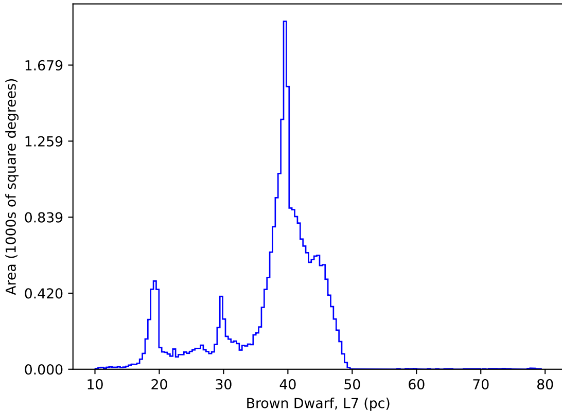
baseline_v3.0_10yrs : Brown Dwarf, L7
