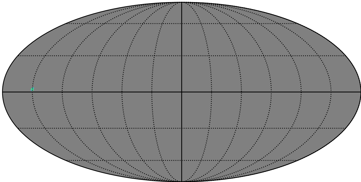
baseline_v3.0_10yrs g band: AGN_TimeLag_5_days
