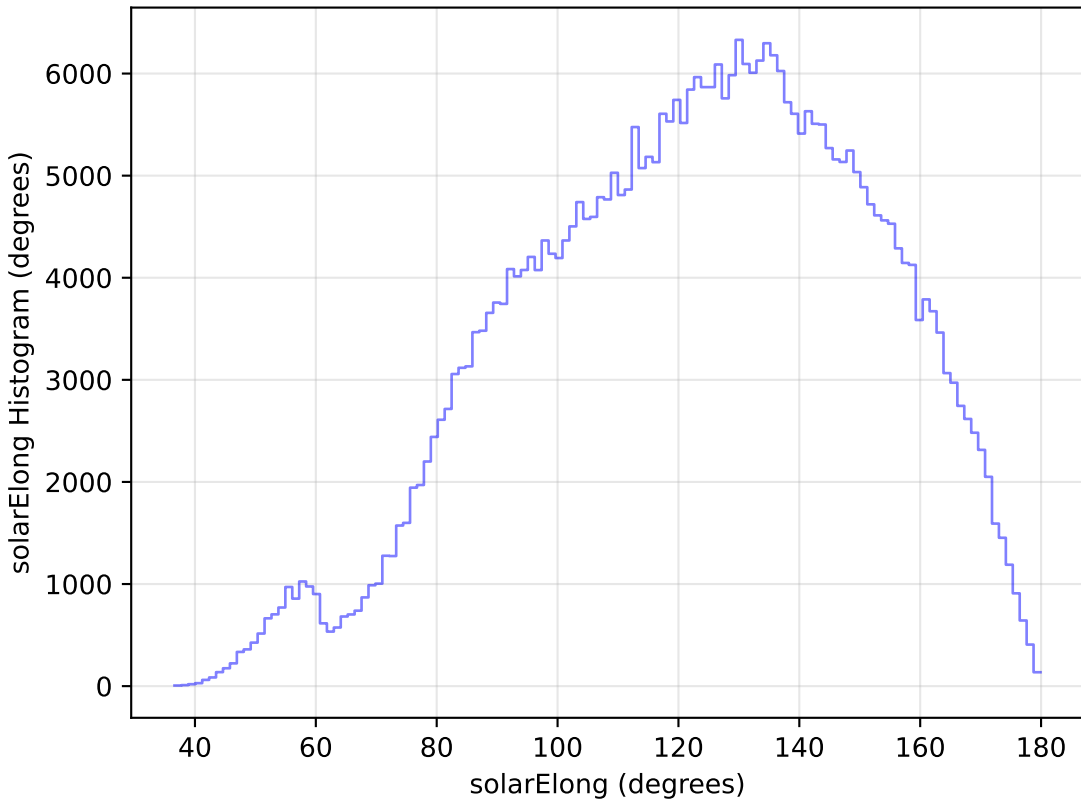
baseline_v3.0_10yrs WFD z band: solarElong Histogram
