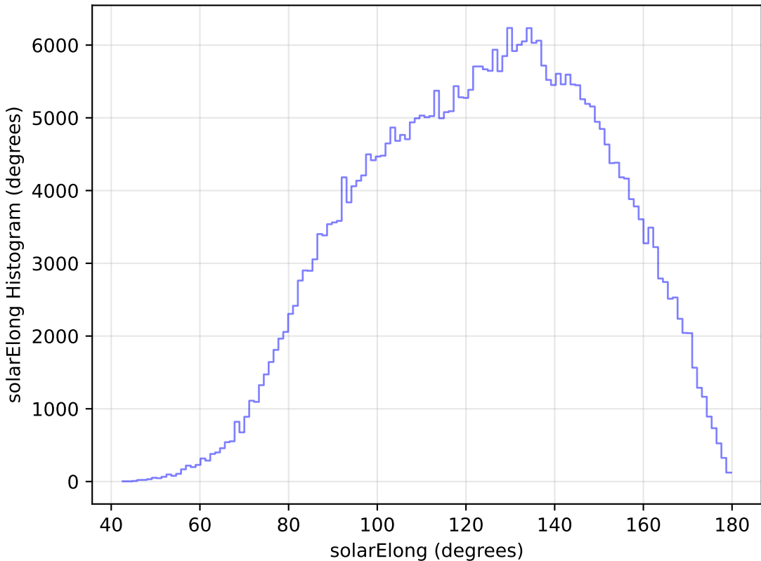
baseline_v3.0_10yrs WFD y band: solarElong Histogram
