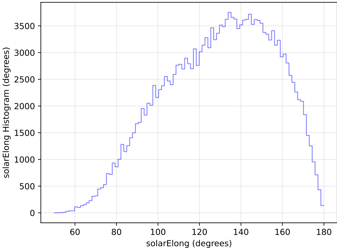
baseline_v3.0_10yrs WFD g band: solarElong Histogram
