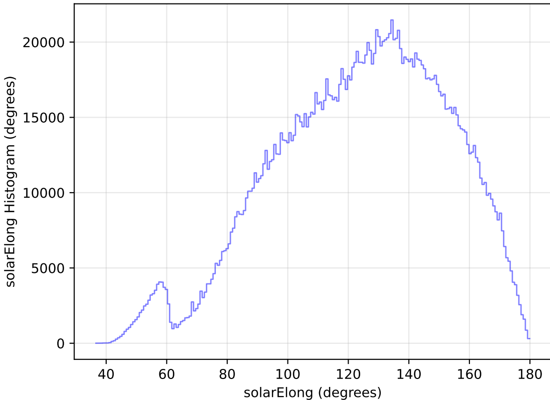
baseline_v3.0_10yrs WFD all bands: solarElong Histogram
