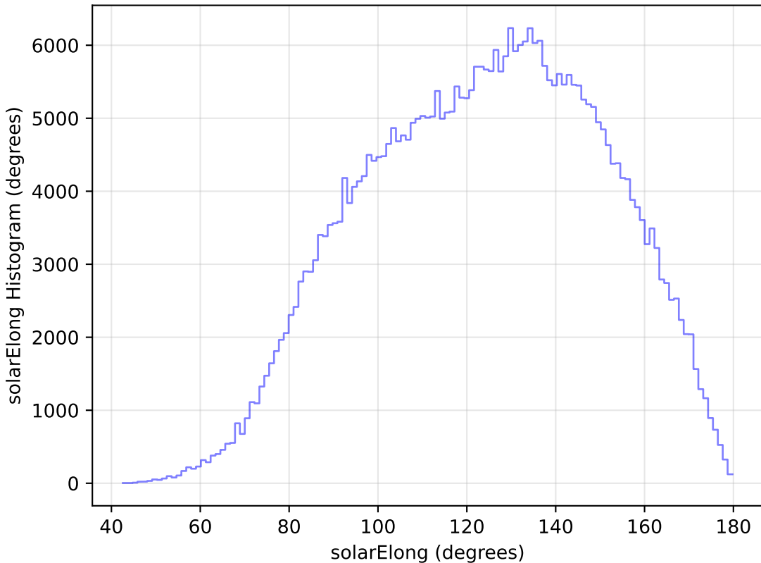
baseline_v3.0_10yrs All sky y band: solarElong Histogram
