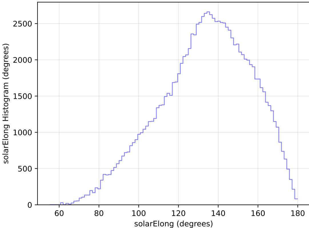
baseline_v3.0_10yrs All sky u band: solarElong Histogram
