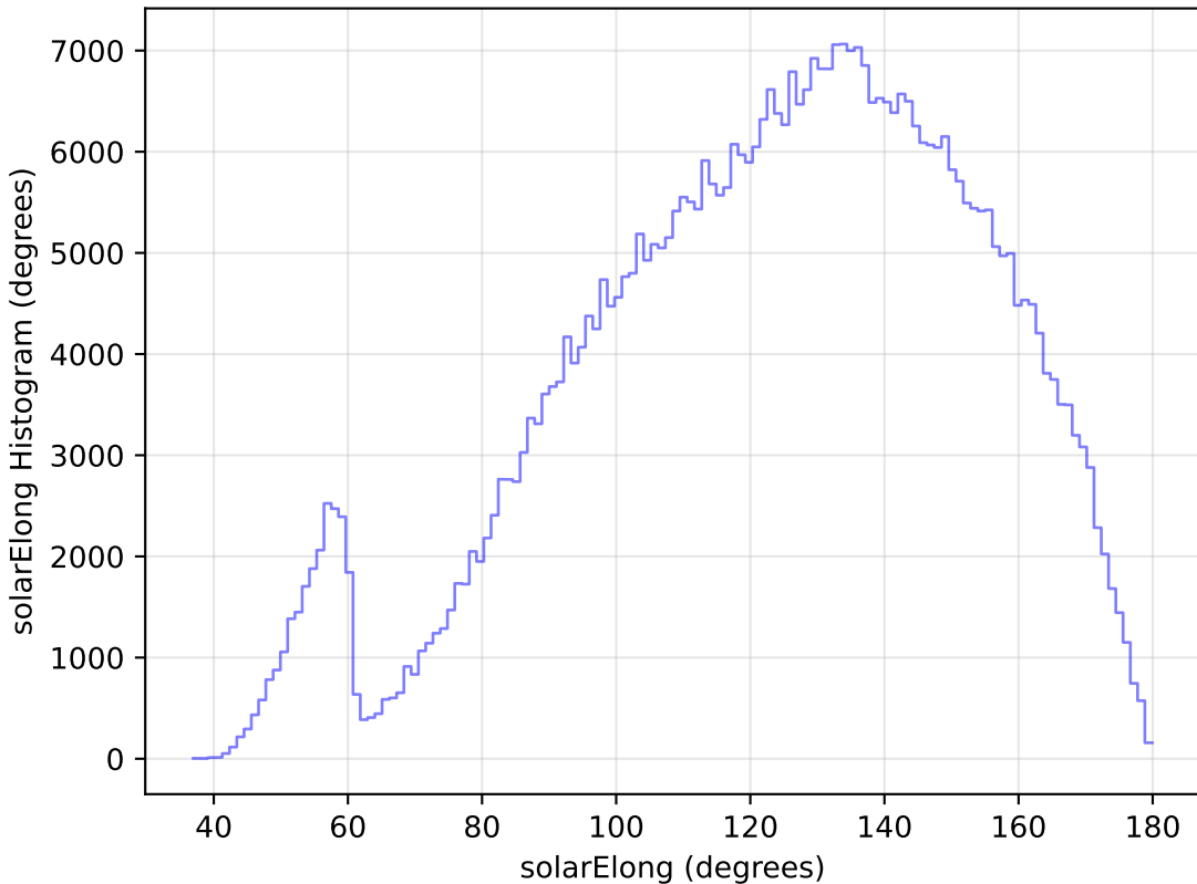
baseline_v3.0_10yrs All sky r band: solarElong Histogram
