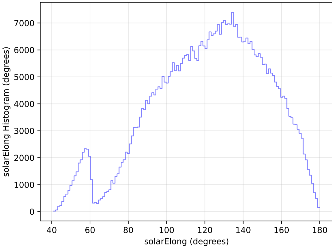
baseline_v3.0_10yrs All sky i band: solarElong Histogram
