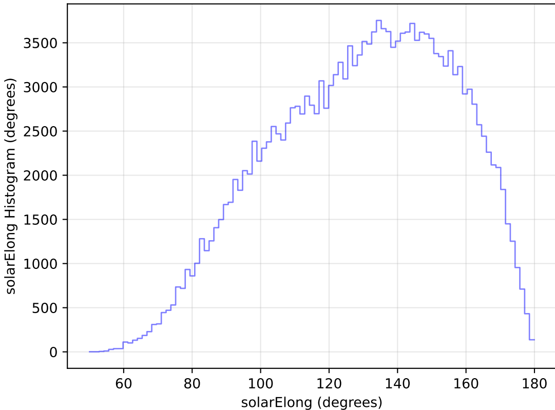
baseline_v3.0_10yrs All sky g band: solarElong Histogram
