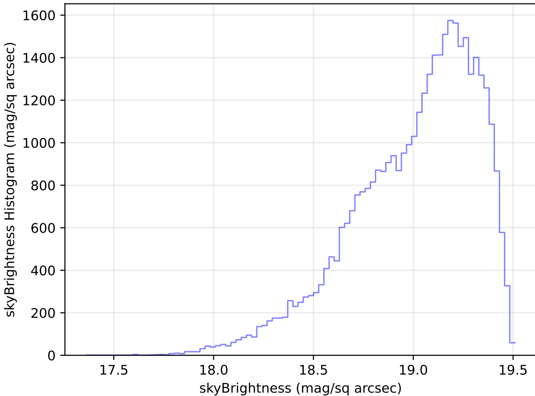
baseline_v3.0_10yrs Yr 1 z band: skyBrightness Histogram
