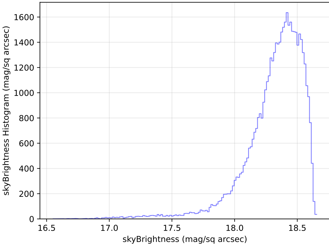
baseline_v3.0_10yrs Yr 1 y band: skyBrightness Histogram
