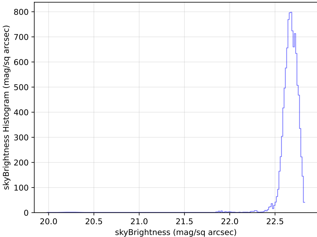
baseline_v3.0_10yrs Yr 1 u band: skyBrightness Histogram
