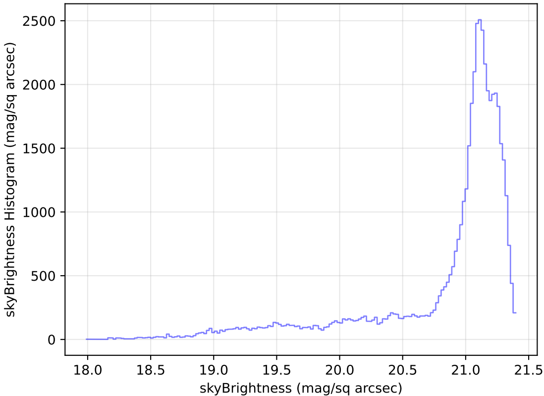
baseline_v3.0_10yrs Yr 1 r band: skyBrightness Histogram
