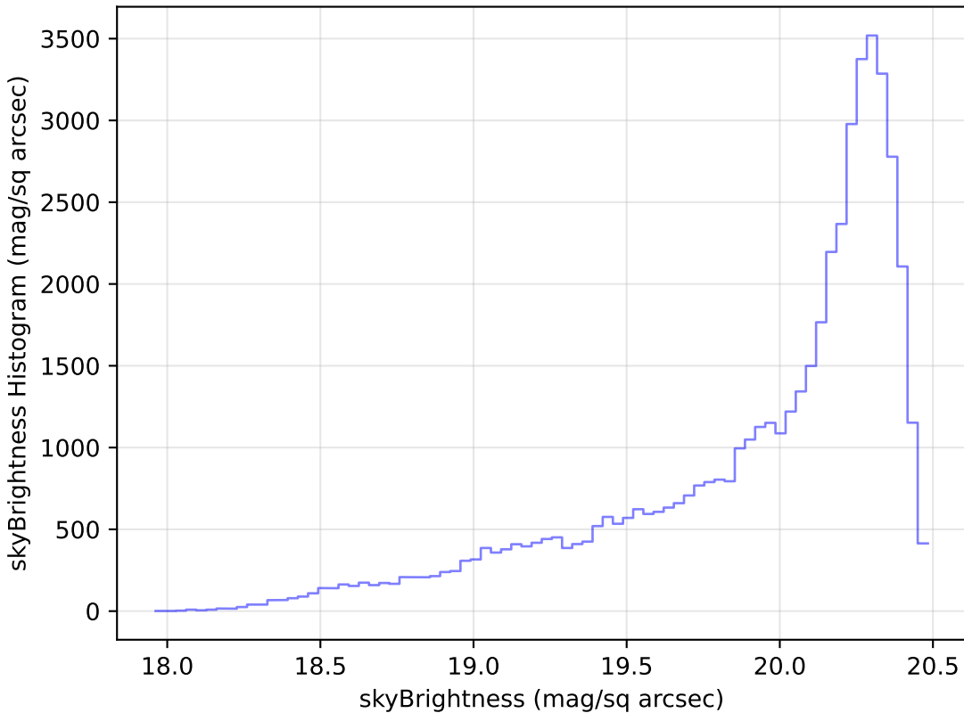
baseline_v3.0_10yrs Yr 1 i band: skyBrightness Histogram
