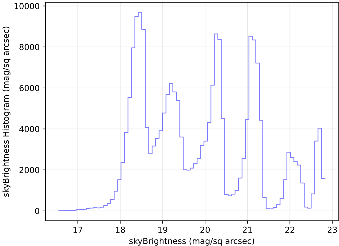
baseline_v3.0_10yrs Yr 1 all bands: skyBrightness Histogram
