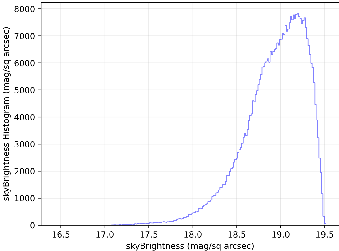
baseline_v3.0_10yrs WFD z band: skyBrightness Histogram
