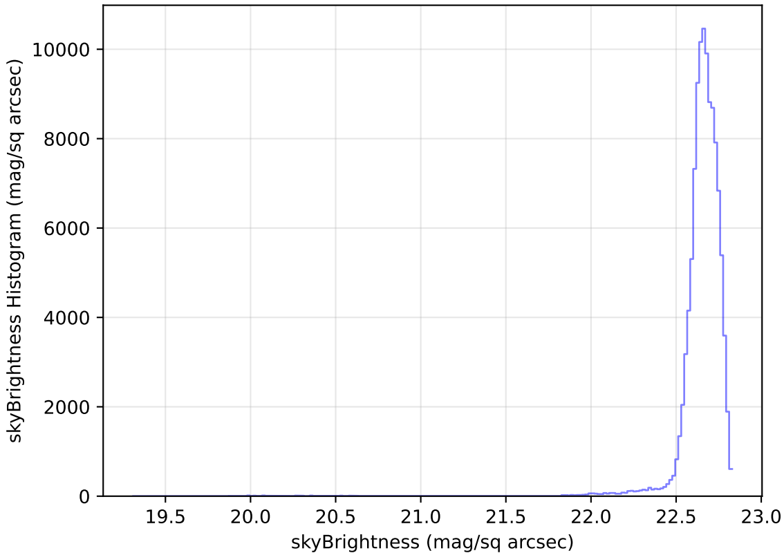
baseline_v3.0_10yrs WFD u band: skyBrightness Histogram
