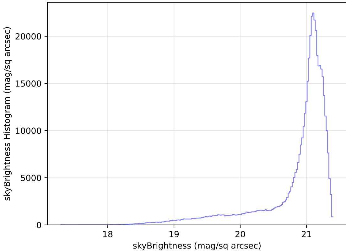
baseline_v3.0_10yrs WFD r band: skyBrightness Histogram
