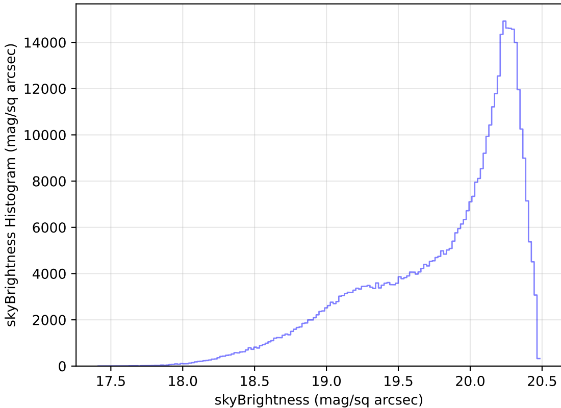
baseline_v3.0_10yrs WFD i band: skyBrightness Histogram
