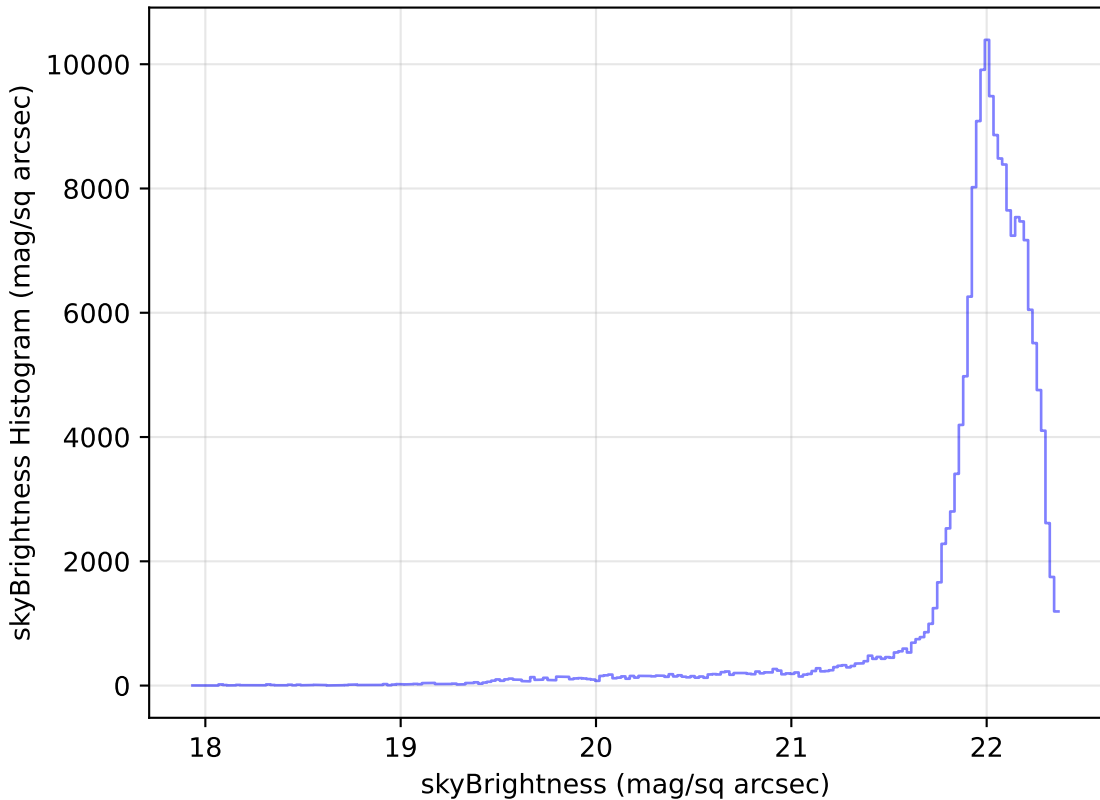
baseline_v3.0_10yrs WFD g band: skyBrightness Histogram
