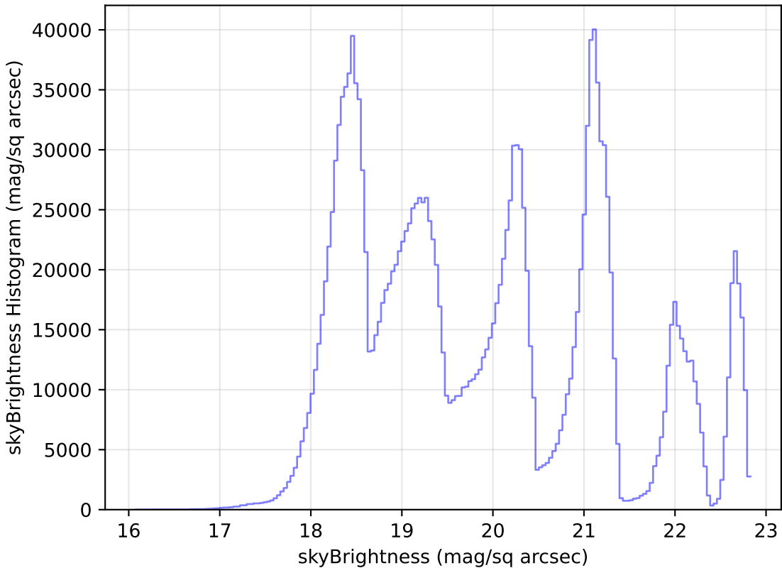
baseline_v3.0_10yrs WFD all bands: skyBrightness Histogram
