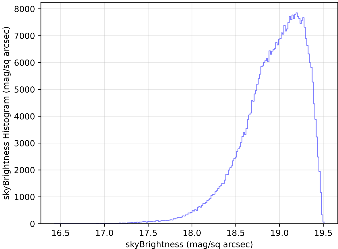
baseline_v3.0_10yrs All sky z band: skyBrightness Histogram
