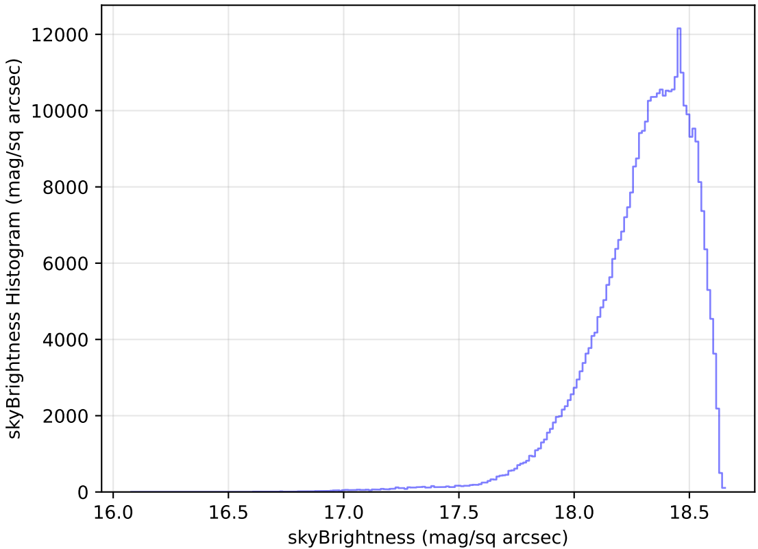
baseline_v3.0_10yrs All sky y band: skyBrightness Histogram
