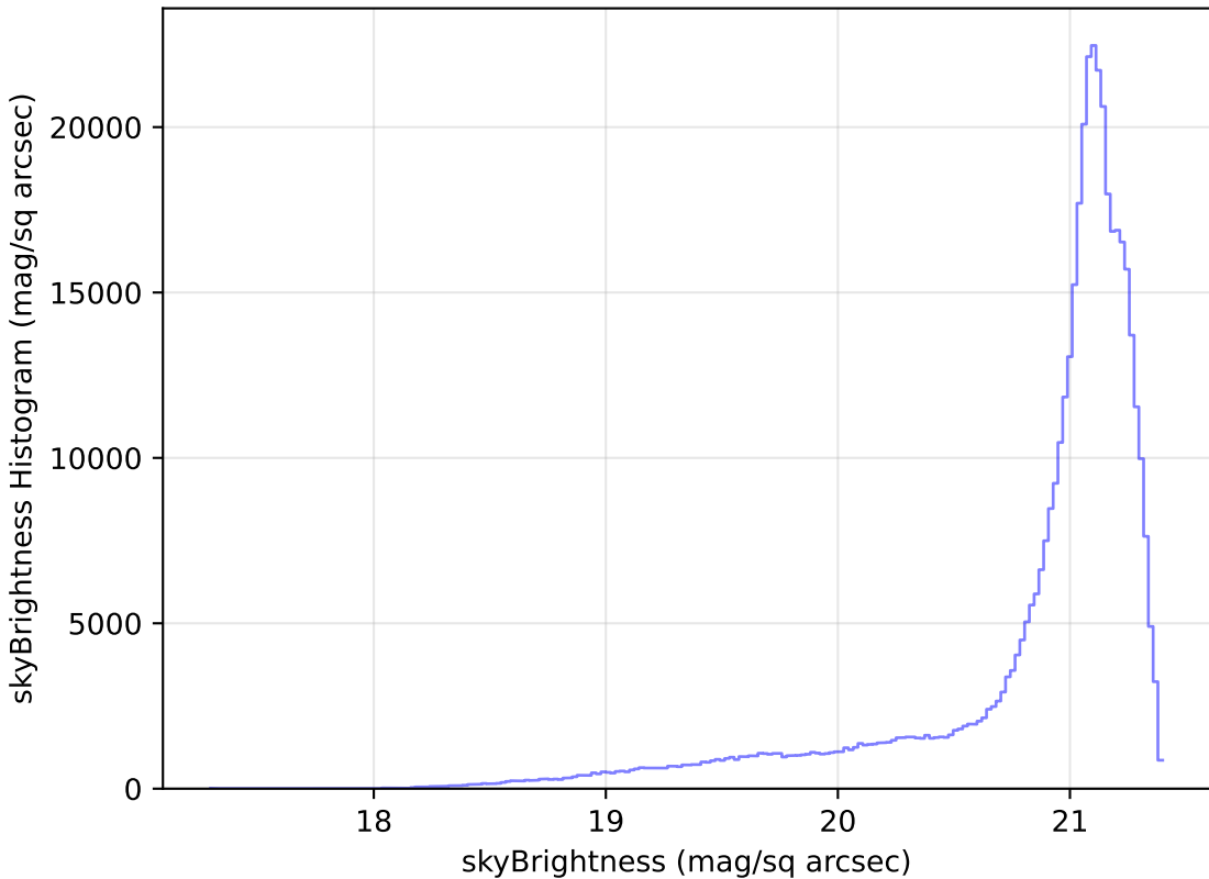
baseline_v3.0_10yrs All sky r band: skyBrightness Histogram
