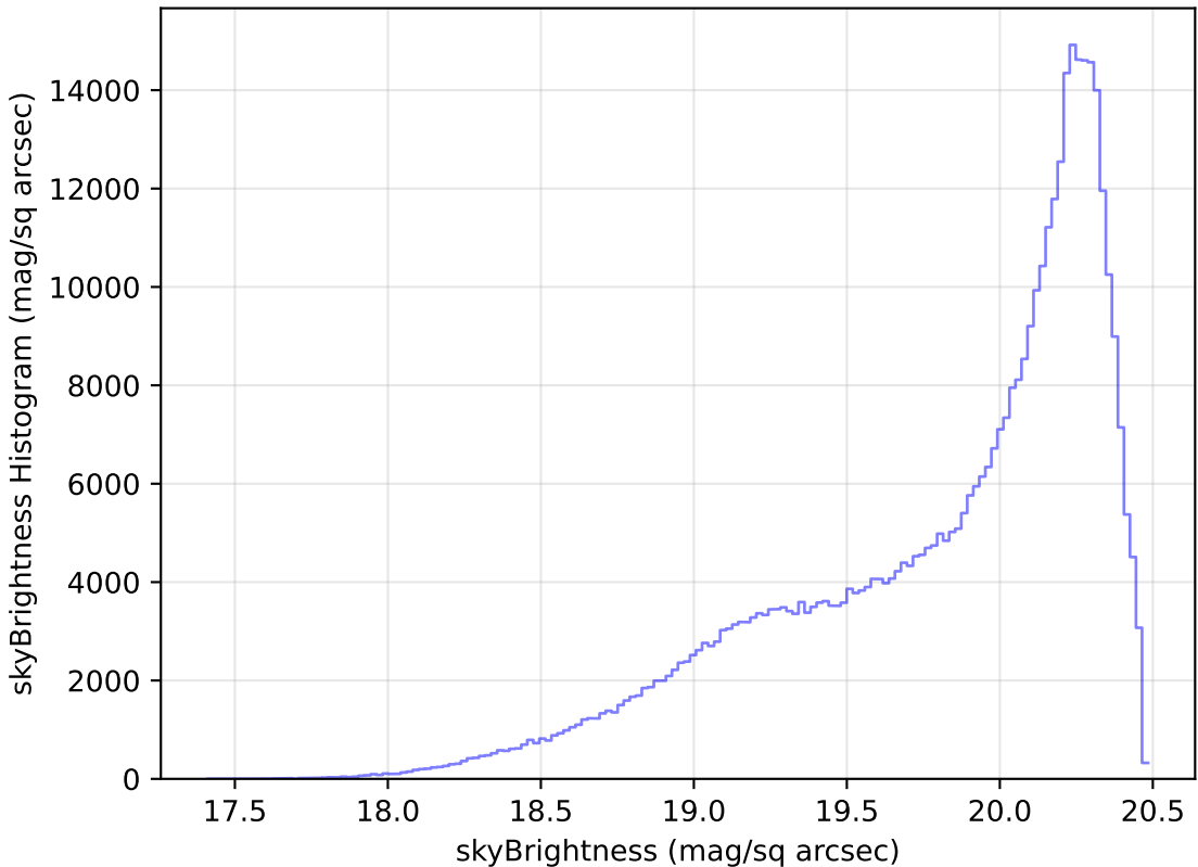
baseline_v3.0_10yrs All sky i band: skyBrightness Histogram
