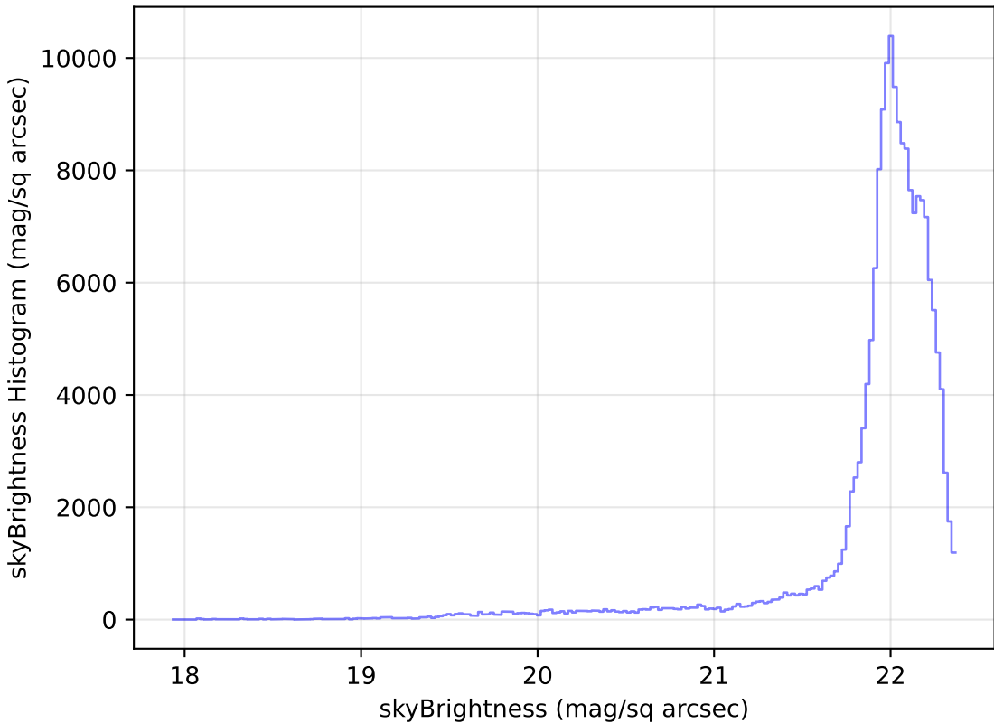
baseline_v3.0_10yrs All sky g band: skyBrightness Histogram
