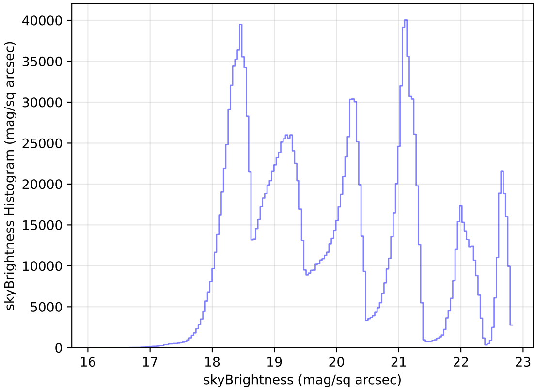
baseline_v3.0_10yrs All sky all bands: skyBrightness Histogram
